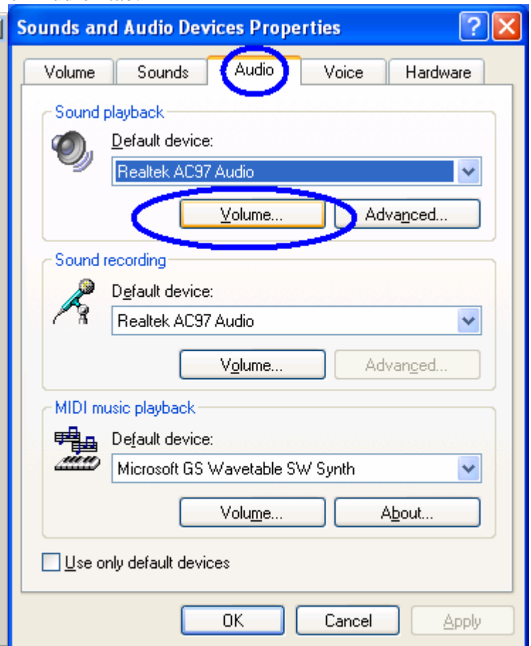
Windows XP
