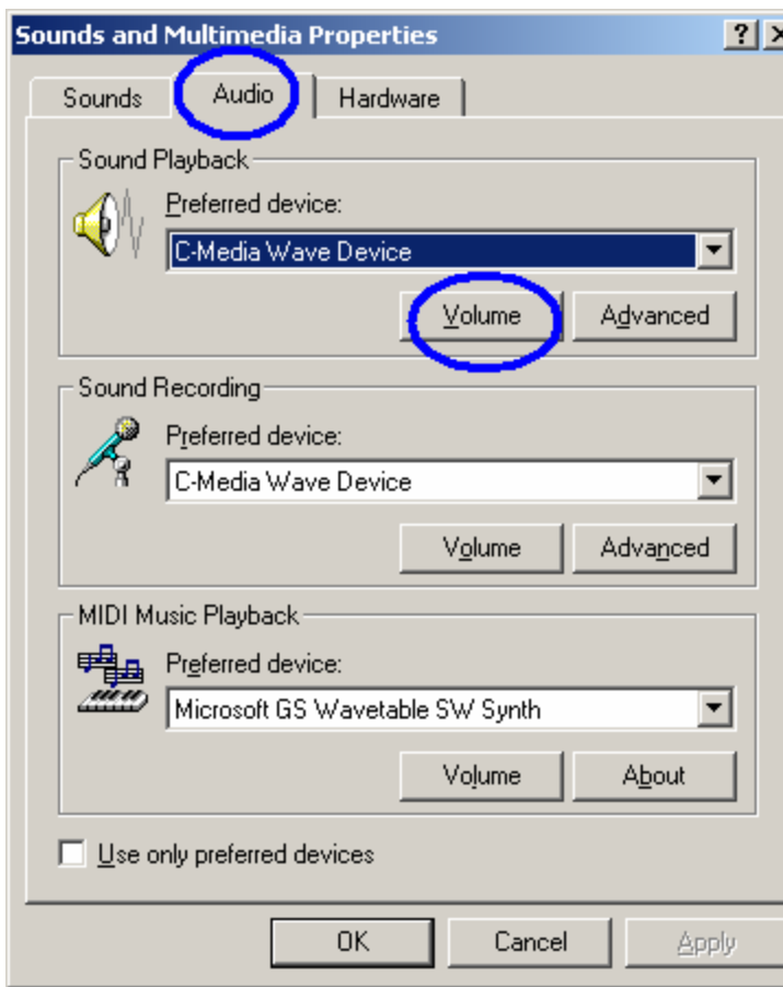
Windows 2000
